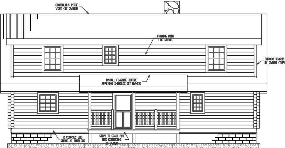
REAR ELEVATION
