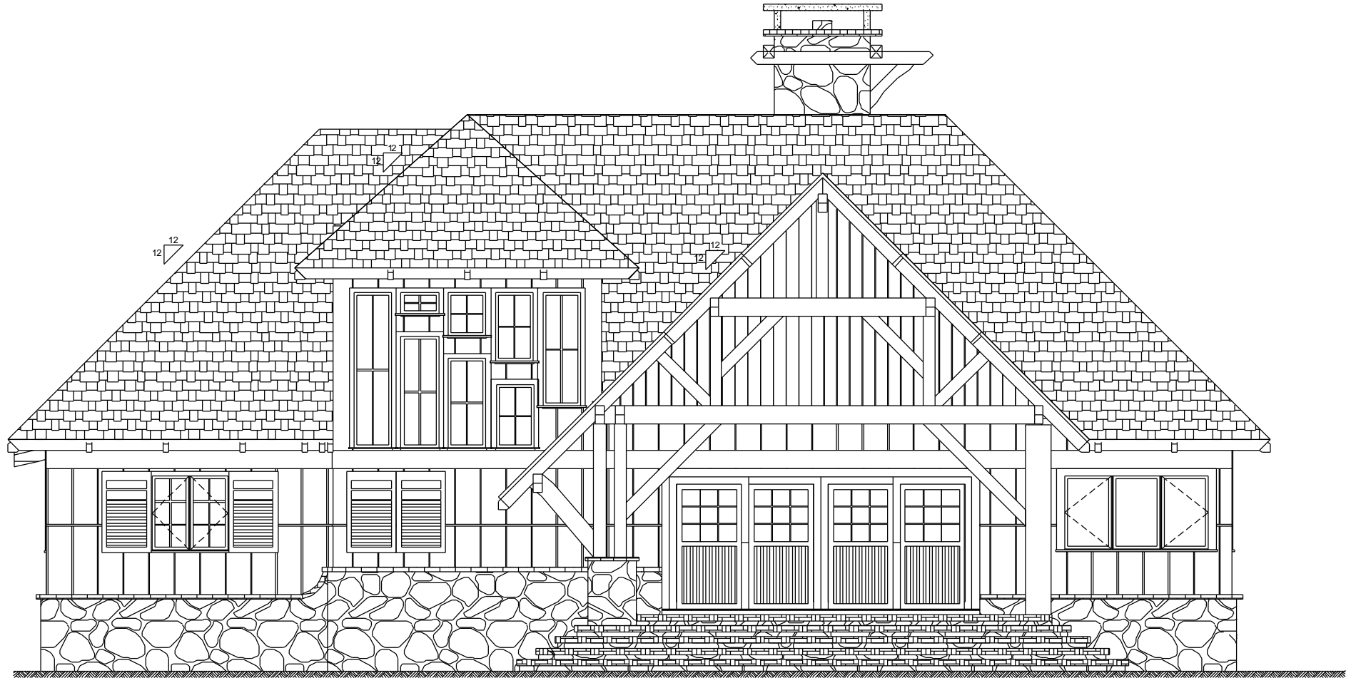
FRONT ELEVATION
