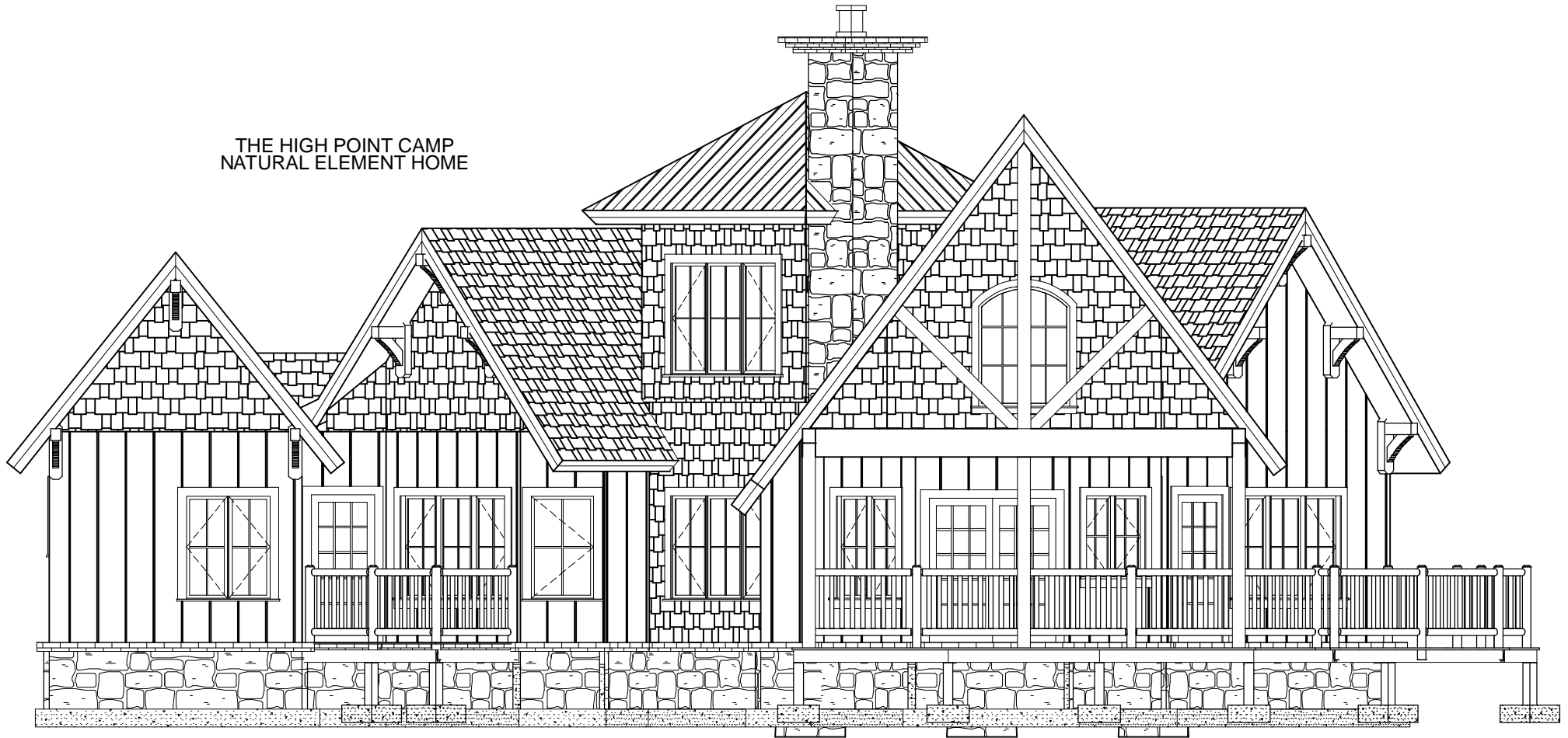
REAR ELEVATION
