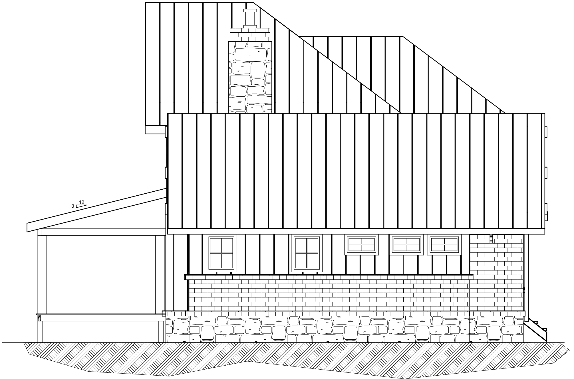
LEFT ELEVATION
