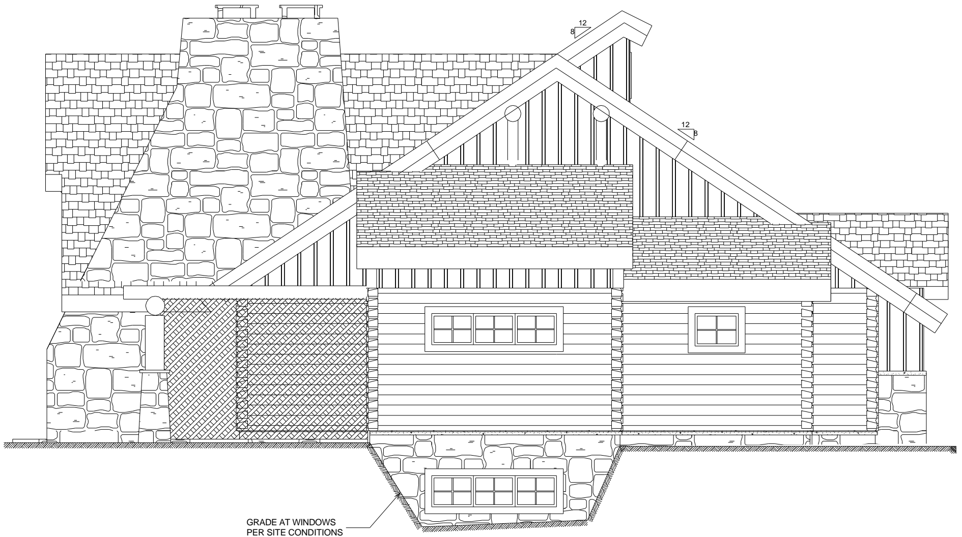
LEFT ELEVATION
